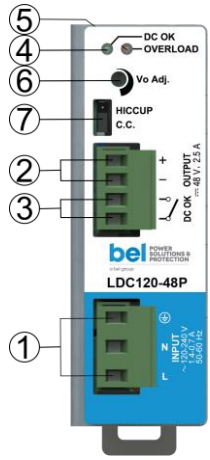
FIG.1 - CONNECTIONS
