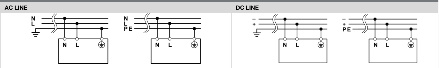
FIG.7 - INPUT CONNECTIONS
