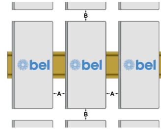
FIG.3 - DISTANCES
