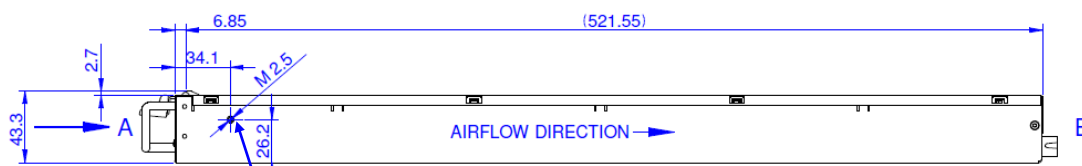
Figure 12. Side view
