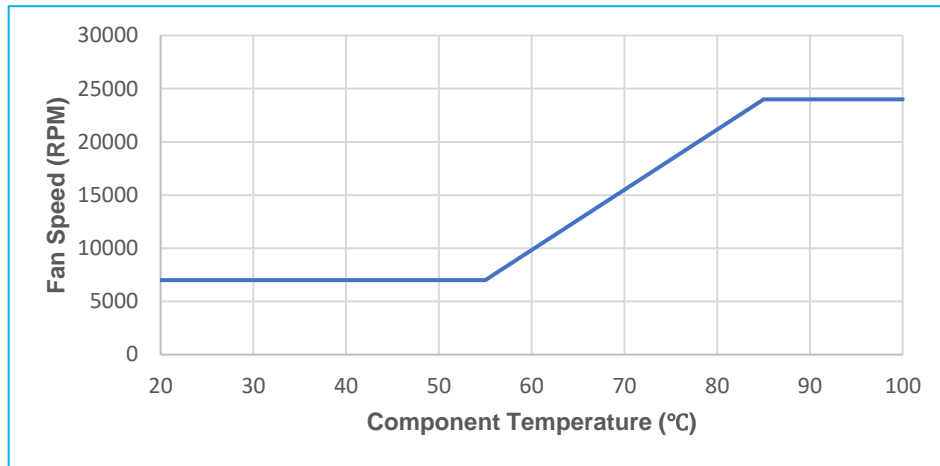
Figure 10. Fan speed versus power stage temperatures
