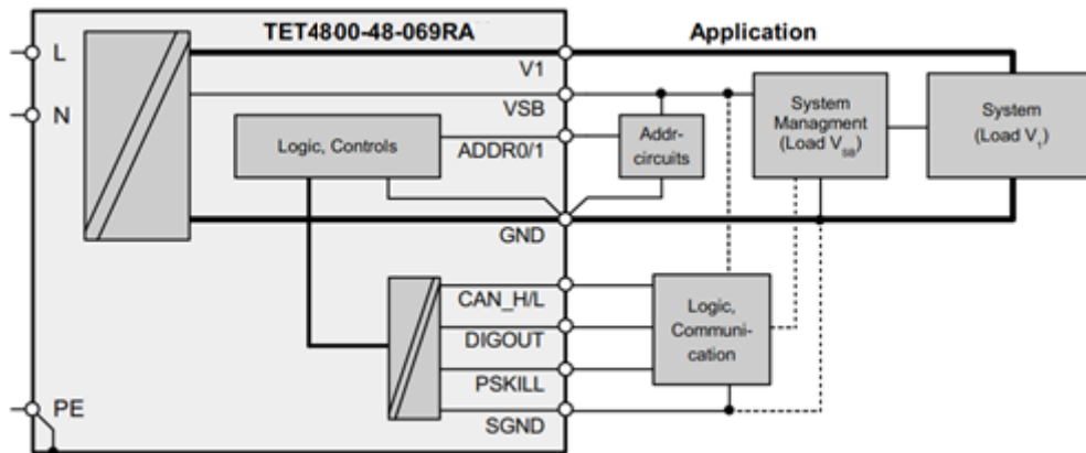
Figure 6. Output connection
