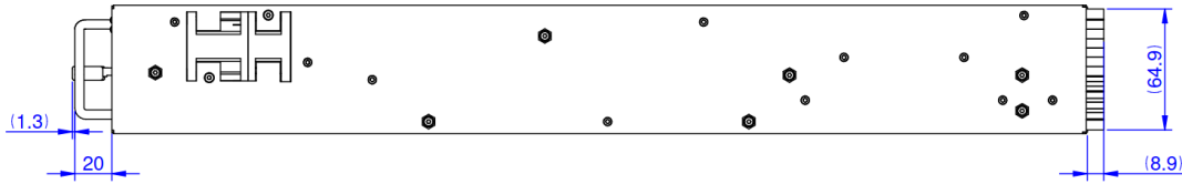
Figure 13. Bottom view
